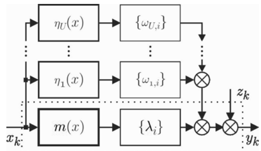
Fig. 6. Uryson system.
